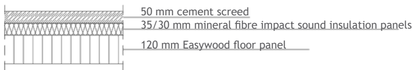
Floor structure 1: Rated standard impact sound level L'_{n,w} = 66 dB
